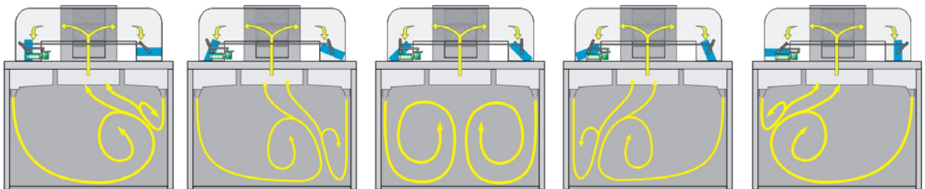
High-Performance Air Handling System
